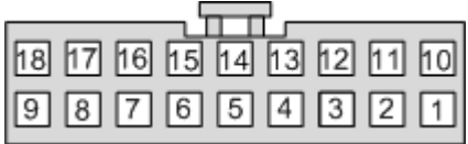
Wire Side
