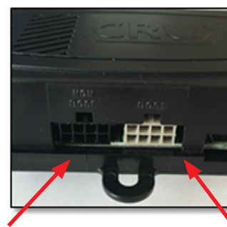
NON BOSE (Non-Amplified) Connection BOSE (Amplified) Connection
